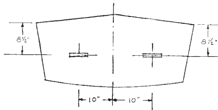
FIGURE 3. LOCATION OF TRANSOM HANDLES--CLASS X
