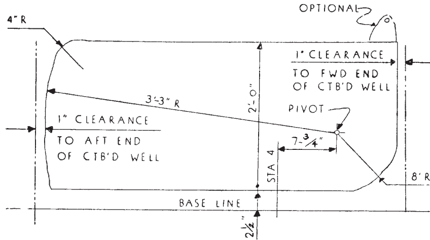
FIGURE 1. CENTERBOARD SHAPE--CLASS X
